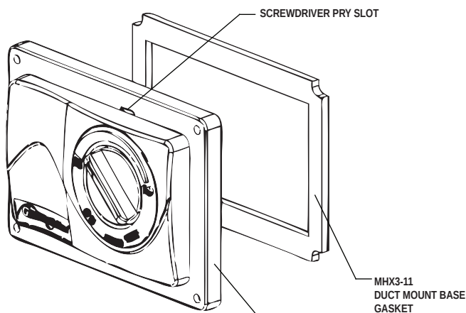
FIG. 2 DUCT MOUNT VERSION
